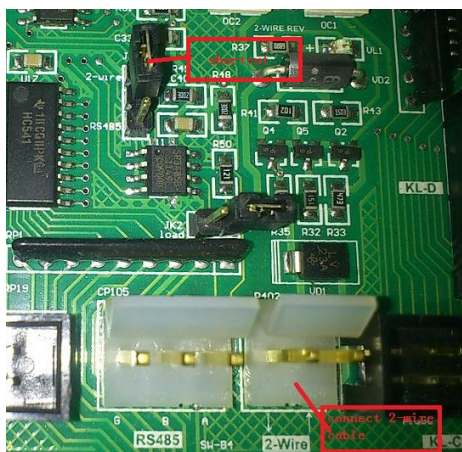
Gilbarco 3202 series dispenser board
