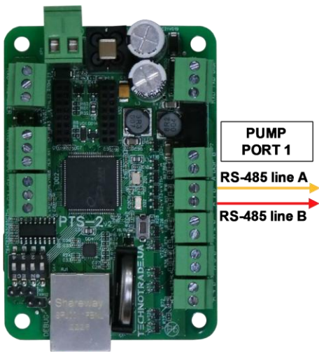
PTS-2 controller
