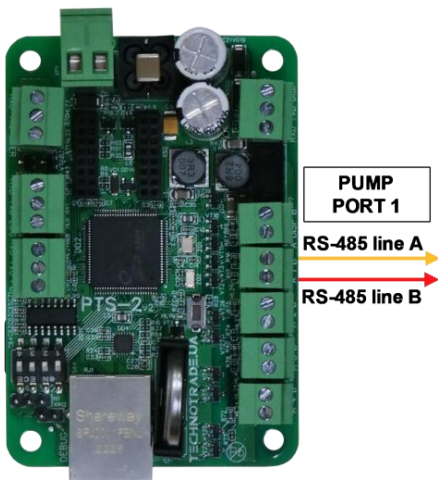
PTS-2 controller
