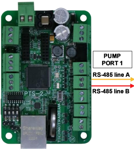
PTS-2 controller
