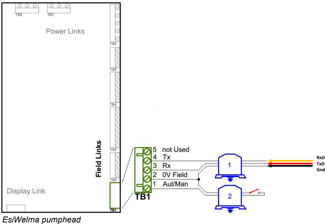
PTS-2 controller
