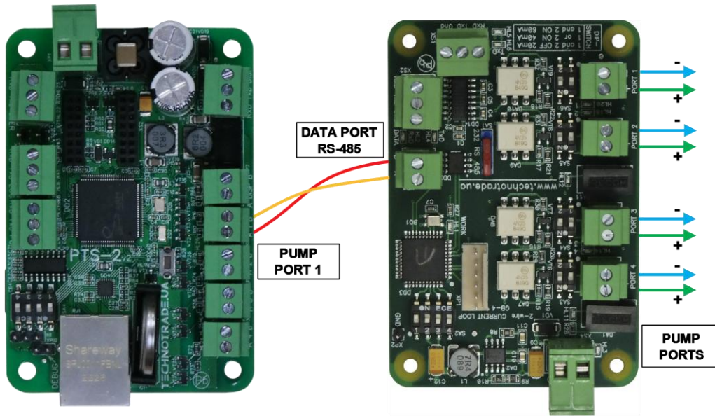
PTS-2 controller
