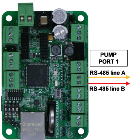
PTS-2 controller
