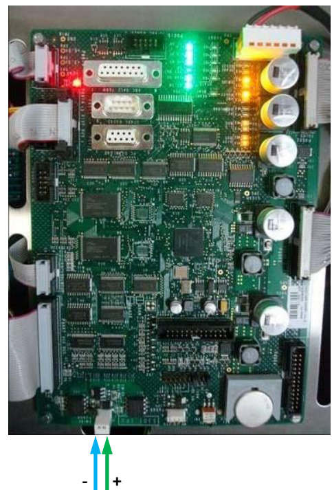
Gilbarco dispenser ASSY M06104A001 rev. B board
