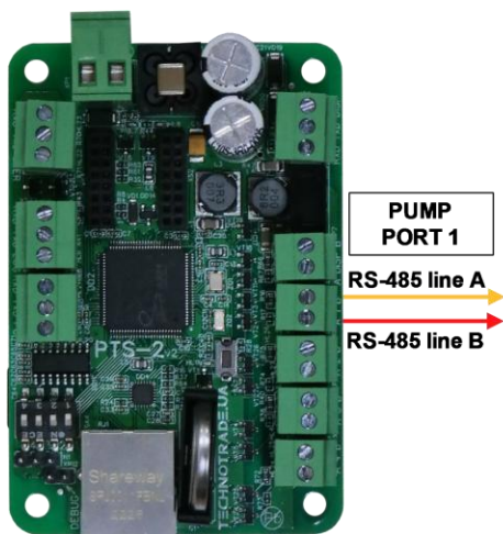
PTS-2 controller
