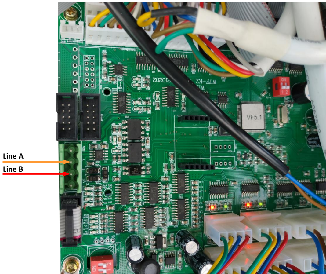
PTS-2 controller
