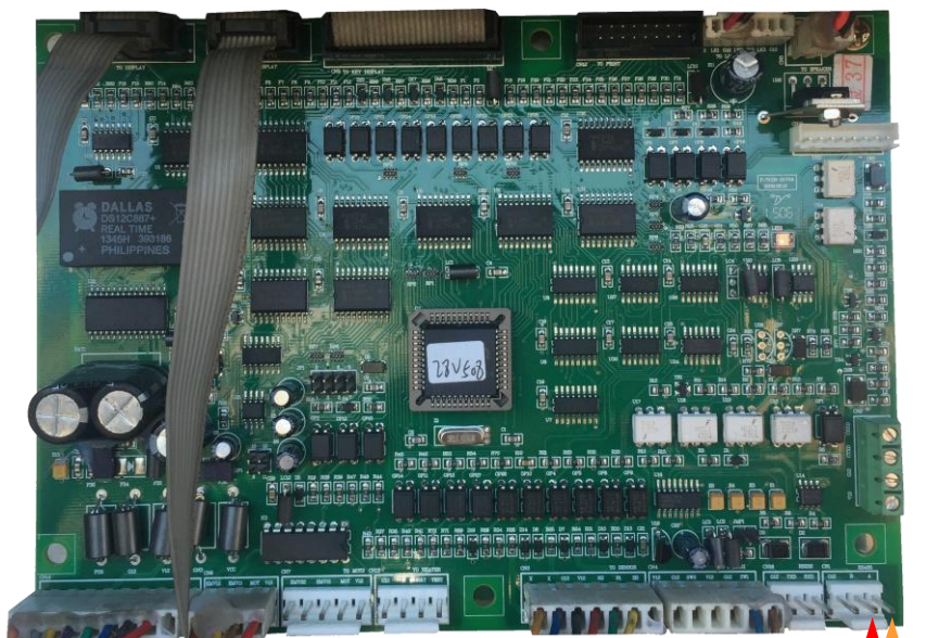
Sanki dispenser board
