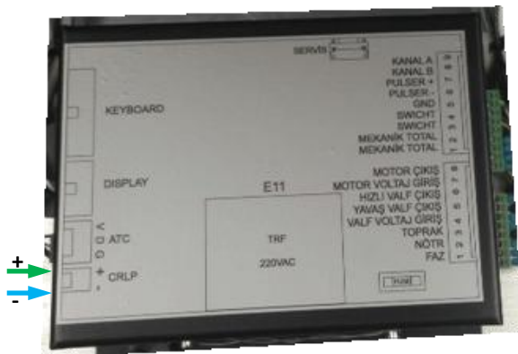
Falcon dispenser computer E11
