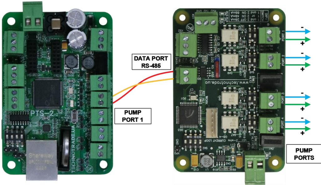
PTS-2 controller
