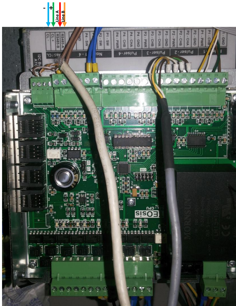
S4s computer
