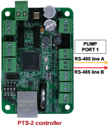
PTS-2 controller
