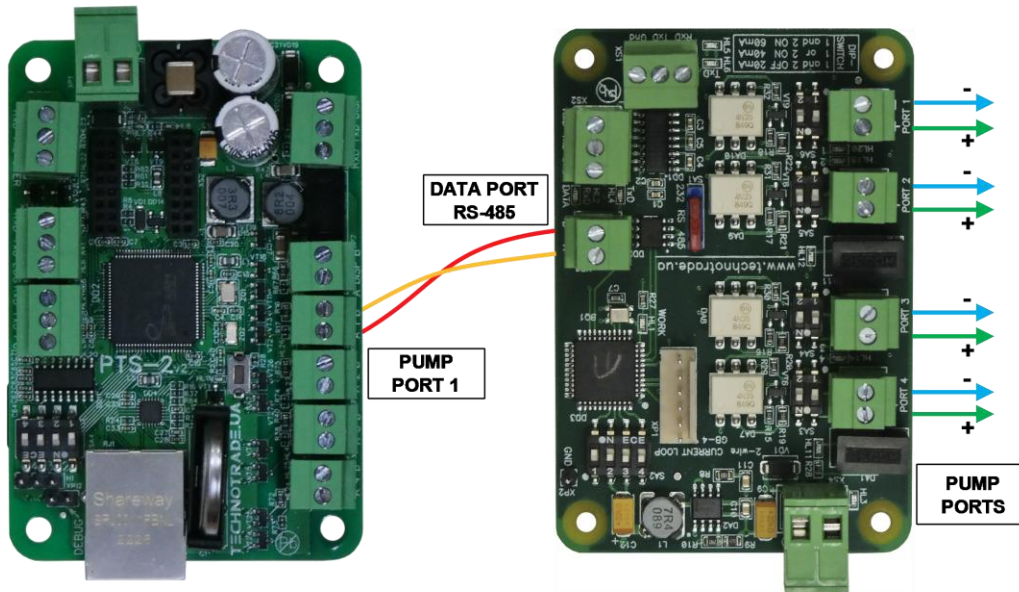
PTS-2 controller
